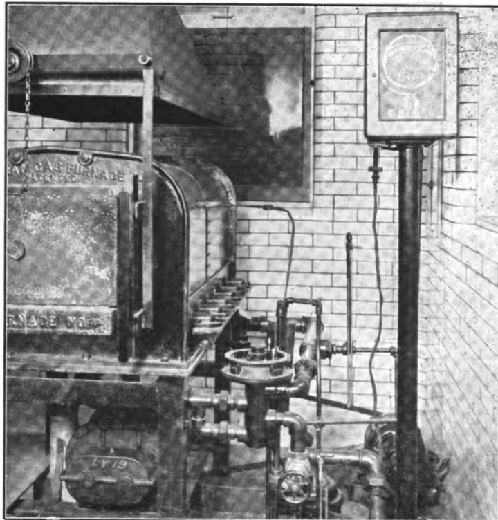
Gas furnace equipped with automatic heat control This device also used for regulating temperatures in japanning ovens—controls temperature to within 5 deg. F.
